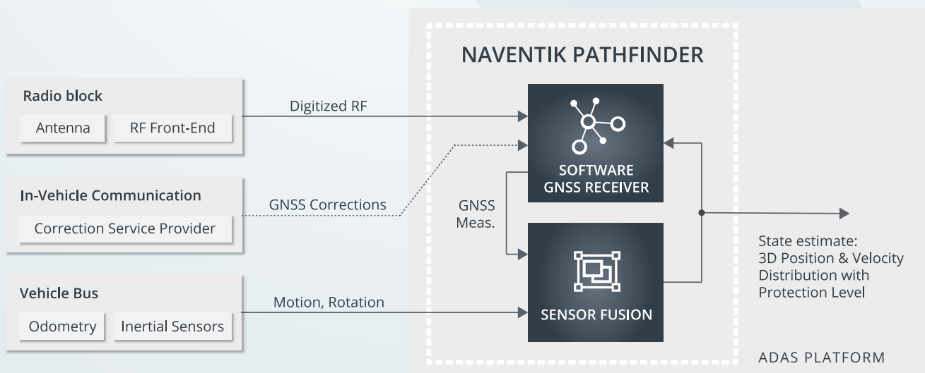
PATHFINDER GNSS+FUSION architecture example
